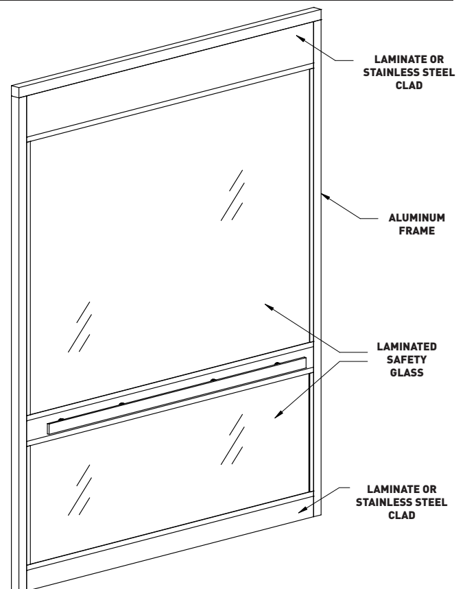
GLASS WALL, ALUMINUM FRAME
