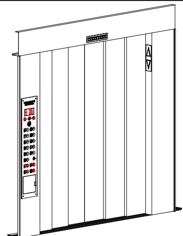
THREE-SPEED CENTER OPENING
